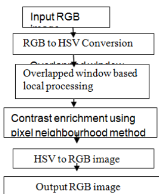
Fig. 1. Flowchart of NTFBLA method
